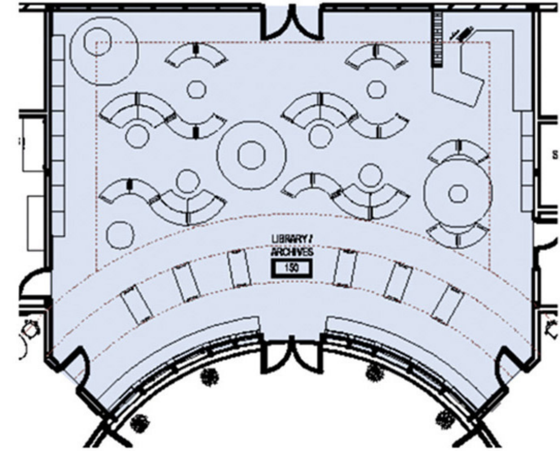
Floor Plan View. Library
